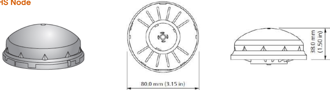
LLC7901/00 SHS Node
